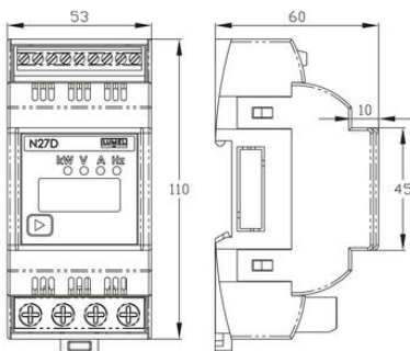
External dimensions
